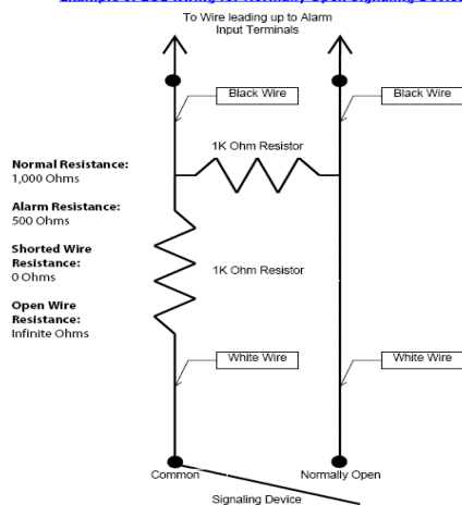
Example of EOL wiring for Normally Open Signaling Device
