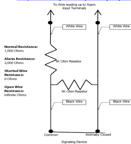
Example of EOL wiring for Normally Closed Signaling Device
