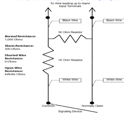
Example of EOL wiring for Normally Open Signaling Device
